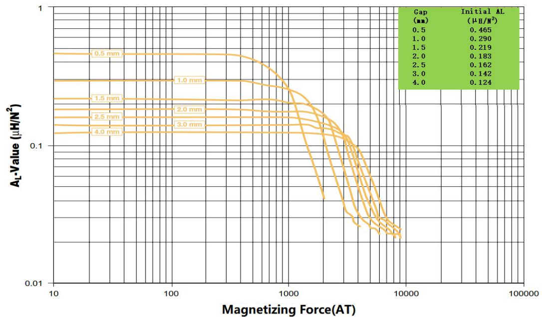
YN-AC-20 Magnetization Curves
