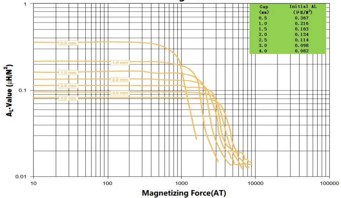
YN-AC-16B Magnetization Curves
